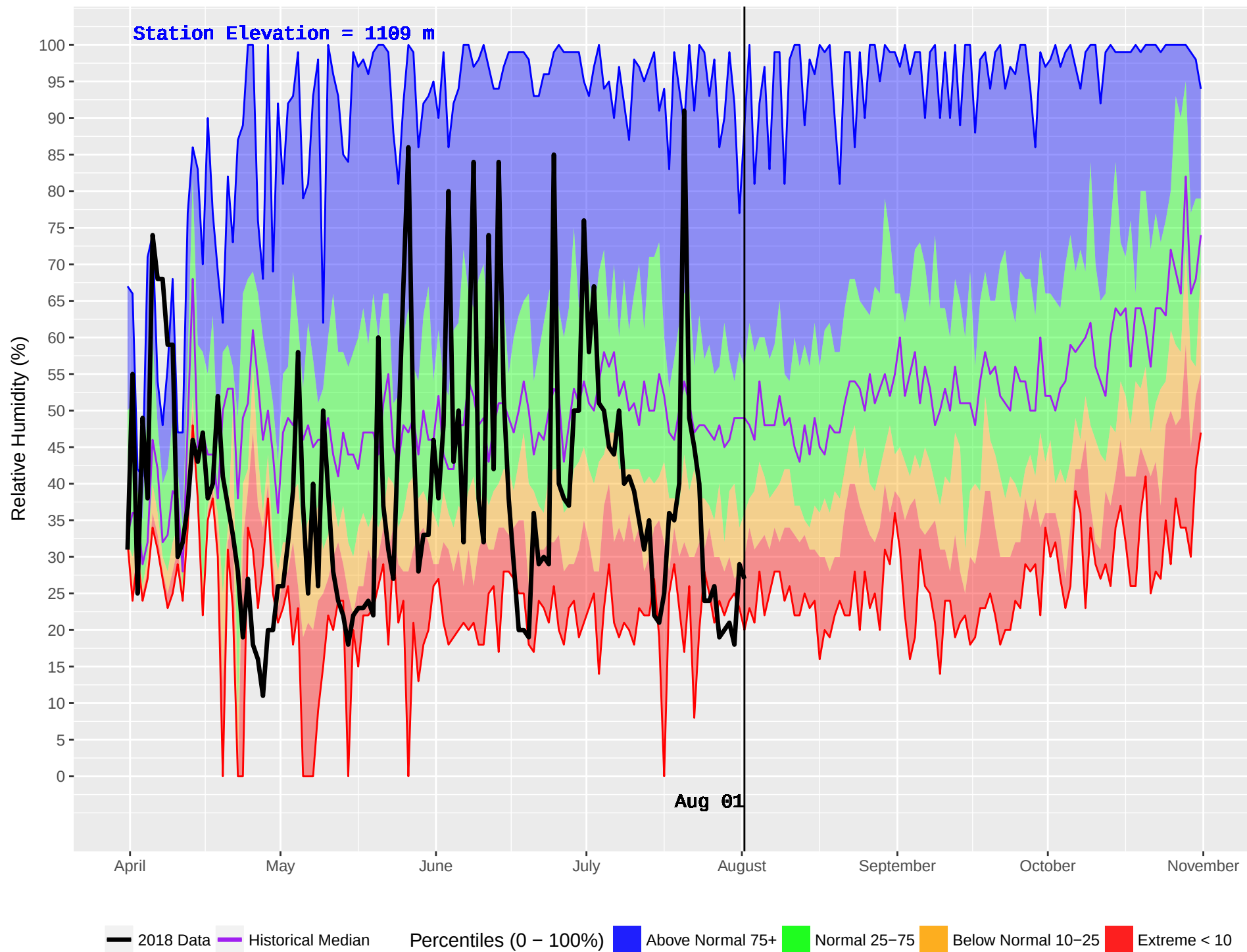
MOOSE LAKE (165) : Historical (1980–2016) and Current (2018) Daily Relative Humidity
