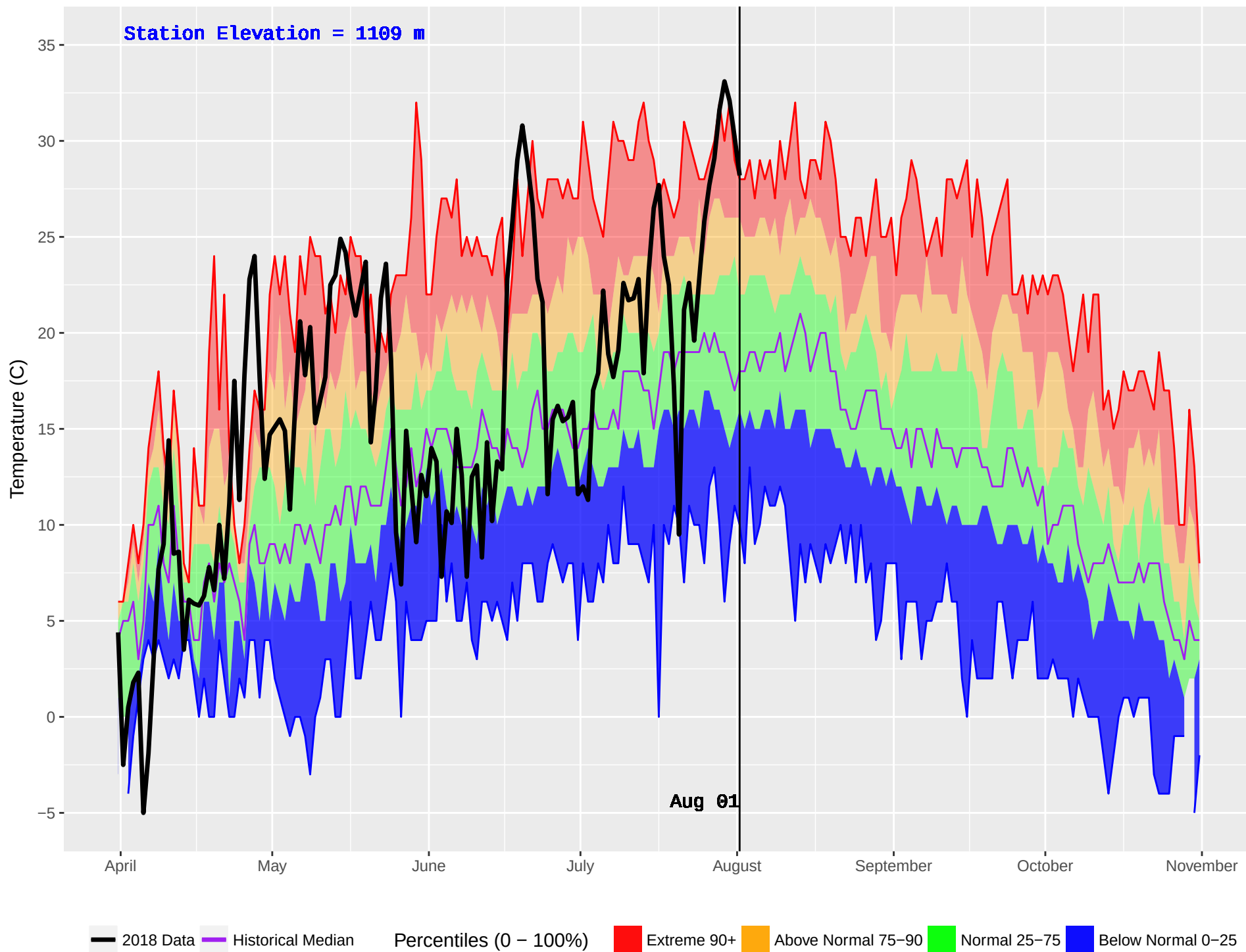
MOOSE LAKE (165) : Historical (1980–2016) and Current (2018) Daily Temperature
