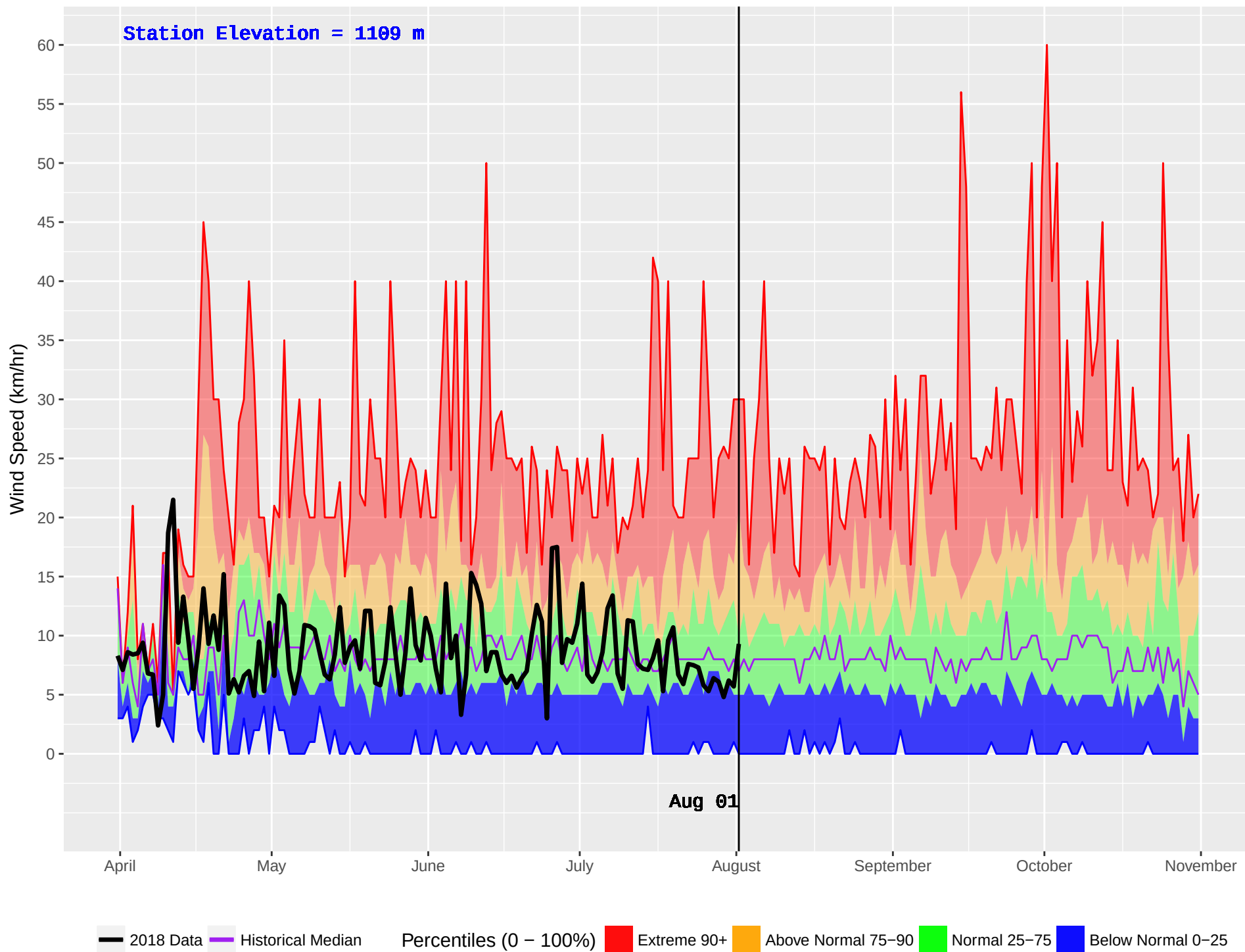
MOOSE LAKE (165) : Historical (1980–2016) and Current (2018) Daily Wind Speed
